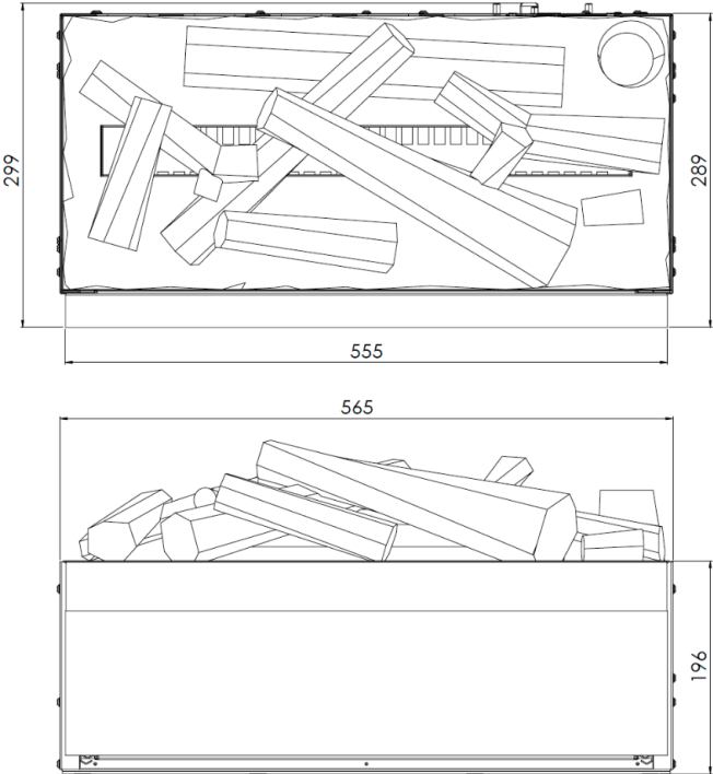
Dimensional Drawing Juneau multi
