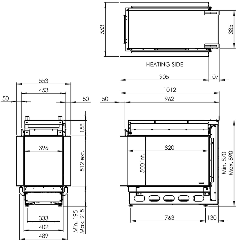
Dimensional Drawing e-Matrix Mood 800/500 RD
