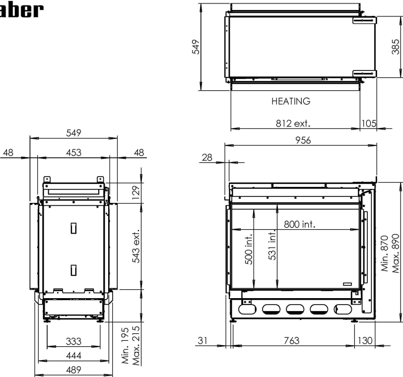
Dimensional Drawing e-MatriX Mood 800/500 ST
