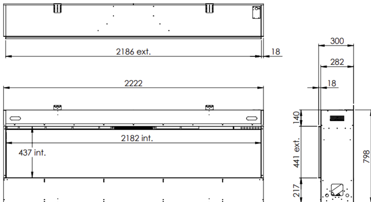
Dimensional drawing e-Slim linear 2200/450 I
